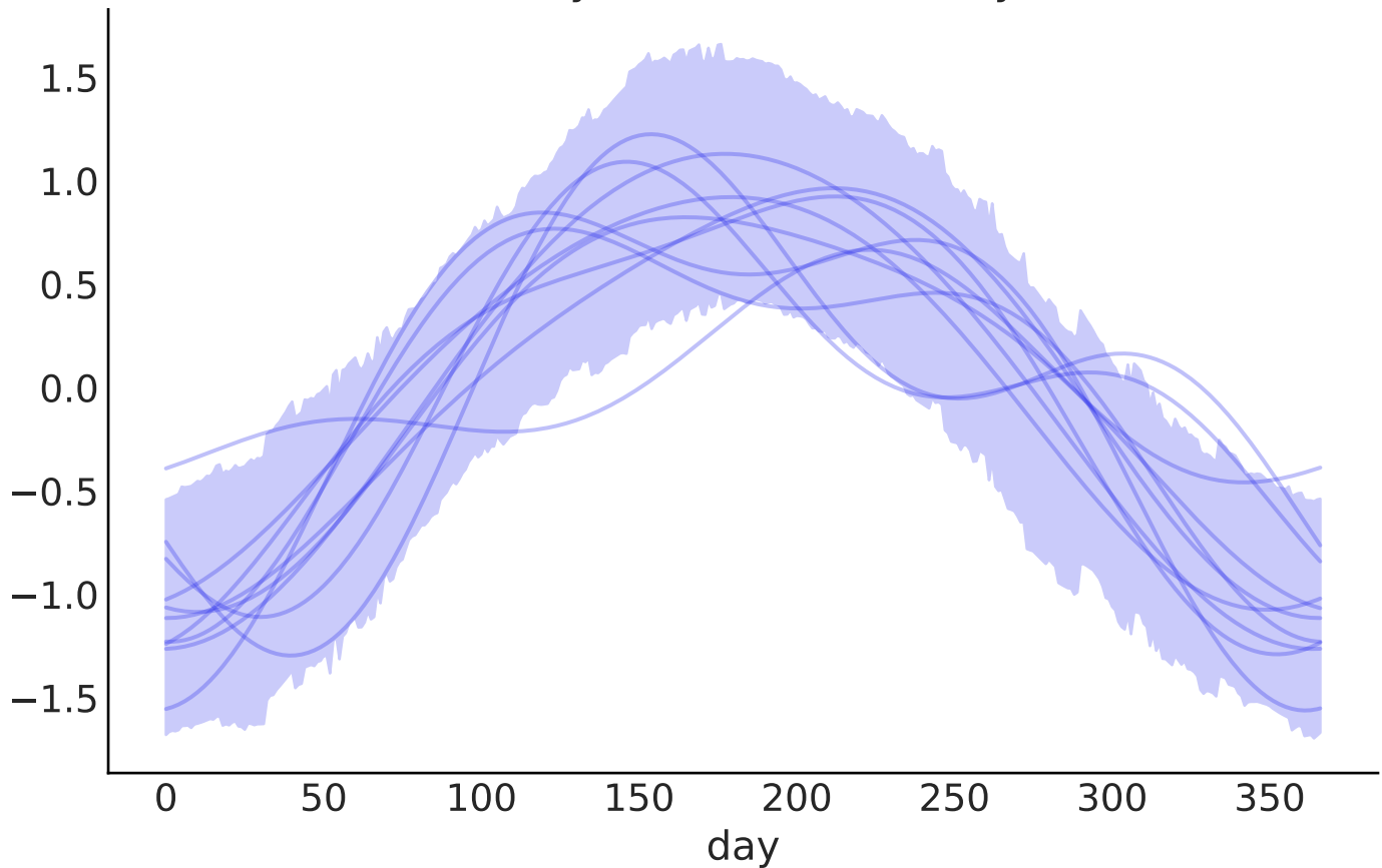
Yearly Fourier Seasonality
